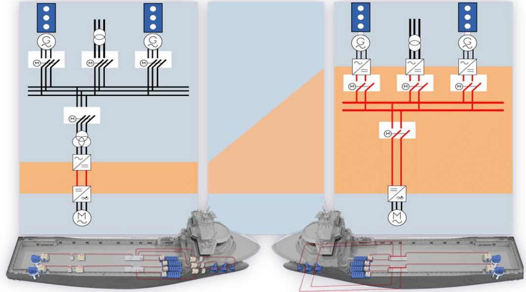
AC Diesel Electric Propulsion
