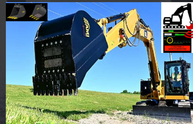
Smart bucket
