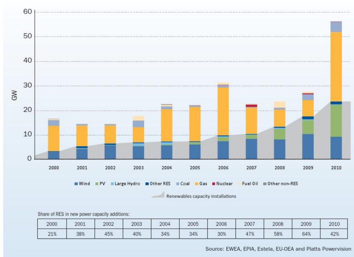
FIGURE 3.5 NEW EU POWER GENERATING CAPACITY (2000 – 2010) – TOTAL 272 GW
