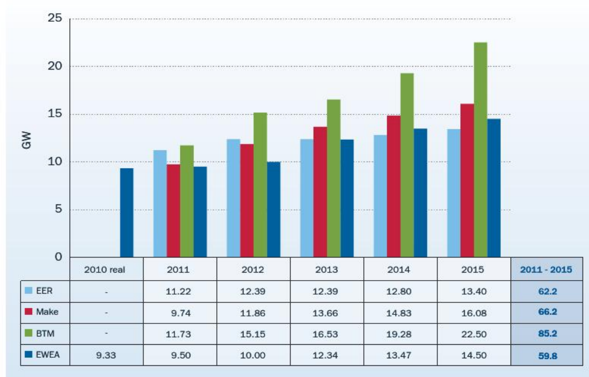
FIGURE 4.4 ANNUAL MARKET FORECASTS (2011 – 2015) EWEA, EER, MAKE CONSULTING AND BTM CONSULT COMPARED
