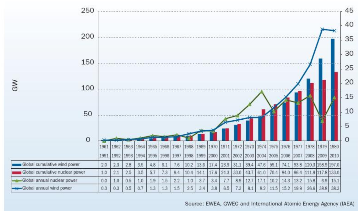
FIGURE 2.3 GLOBAL WIND POWER DEVELOPMENT (1991 – 2010) COMPARED TO NUCLEAR DEVELOPMENT (1961-1980)
