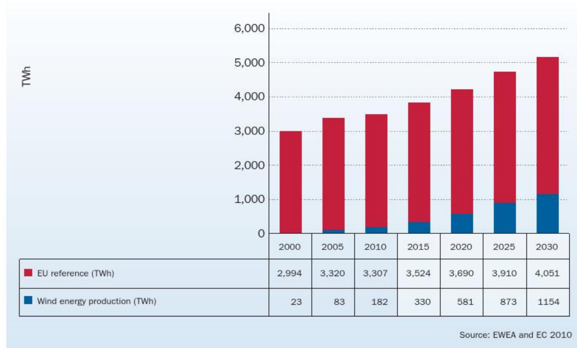
FIGURE 7.1 WIND ENERGY SHARE OF EU ELECTRICITY DEMAND (2000 - 2030)
