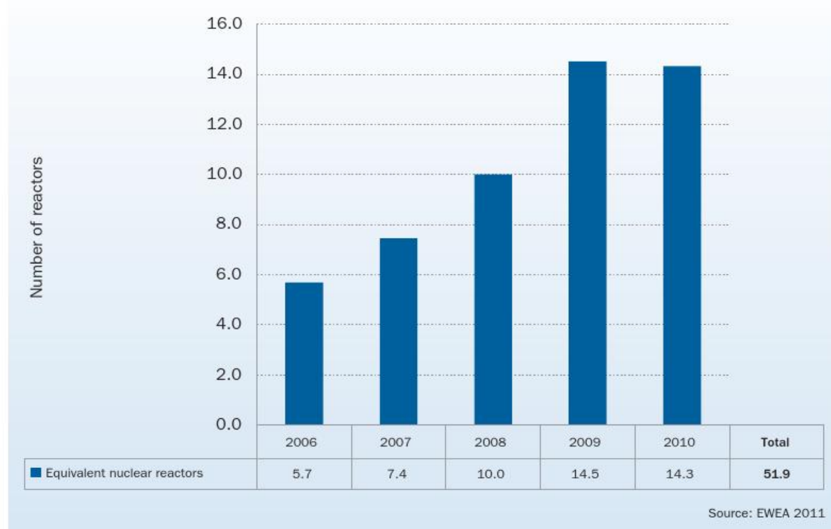
FIGURE 2.6 POWER PRODUCTION FROM ANNUAL GLOBAL WIND CAPACITY ADDITIONS 2006-2010 IN NUCLEAR REACTOR ELECTRICITY EQUIVALENTS
