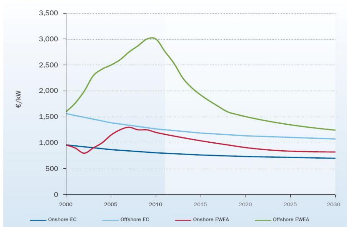
FIGURE 10.1 CAPITAL COST OF ONSHORE AND OFFSHORE WIND
