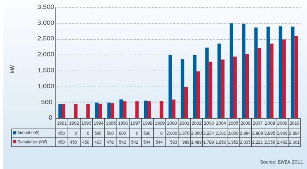
FIGURE 2.15 AVERAGE CAPACITY OF EUROPEAN OFFSHORE WIND TURBINES, ANNUAL AND CUMULATIVE
