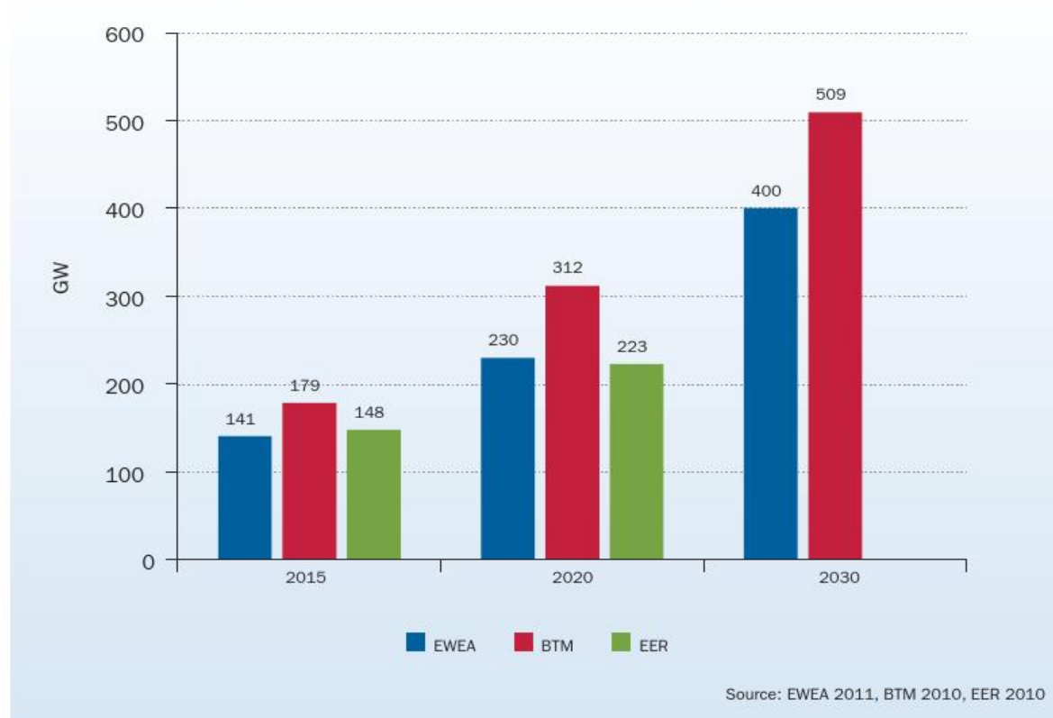
FIGURE 6.2 TOTAL INSTALLED WIND POWER CAPACITY IN EUROPE – EWEA, BTM AND EER SCENARIOS COMPARED
