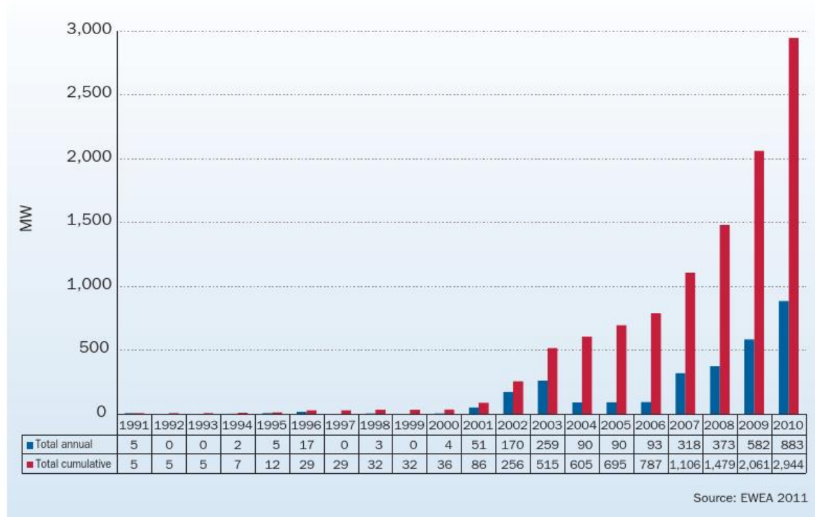
FIGURE 2.10 ANNUAL AND CUMULATIVE INSTALLED EU OFFSHORE CAPACITY 1991-2010 (MW)
