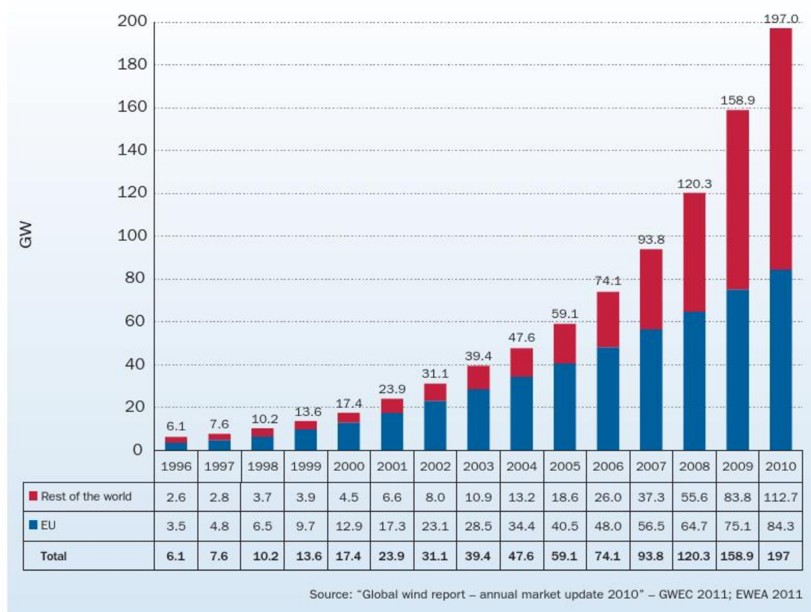
FIGURE 2.1 GLOBAL CUMULATIVE WIND POWER CAPACITY (1996 – 2010)
