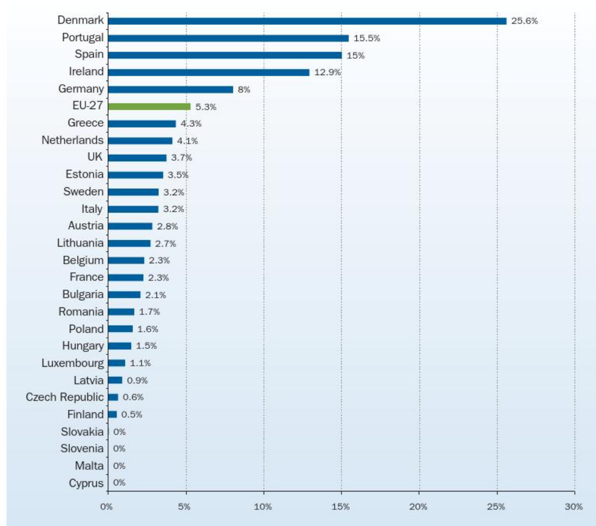
FIGURE 2.11 WIND ENERGY'S SHARE OF NATIONAL ELECTRICITY DEMAND AT END 2010
