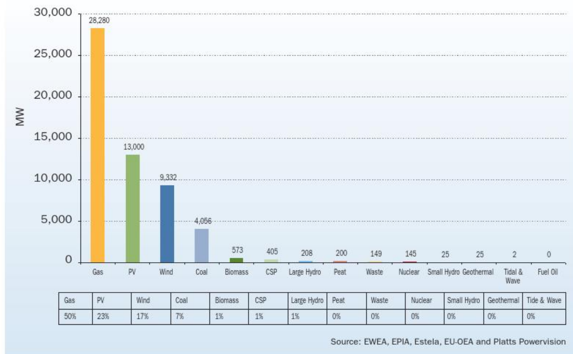
FIGURE 3.7 NEW INSTALLED POWER CAPACITY 2010 – TOTAL 56,400 MW
