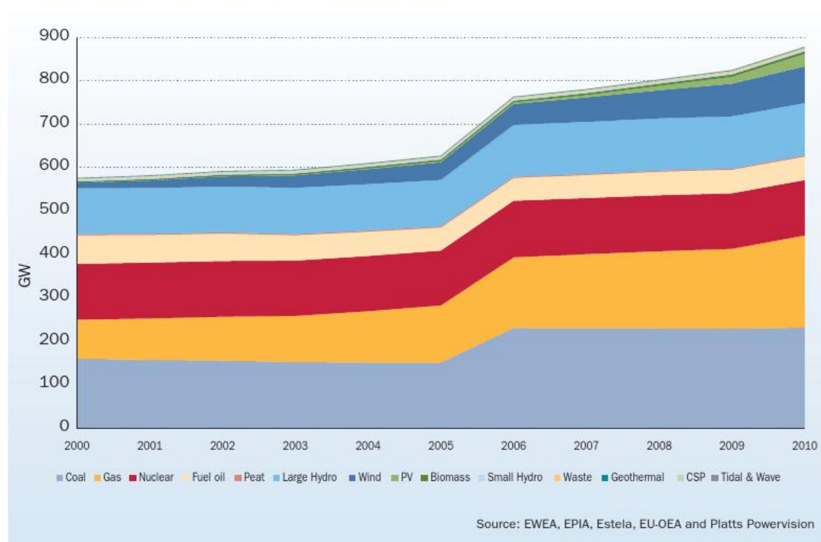
FIGURE 3.1 INSTALLED POWER CAPACITY (GW) IN THE EU (2000 – 2010)
