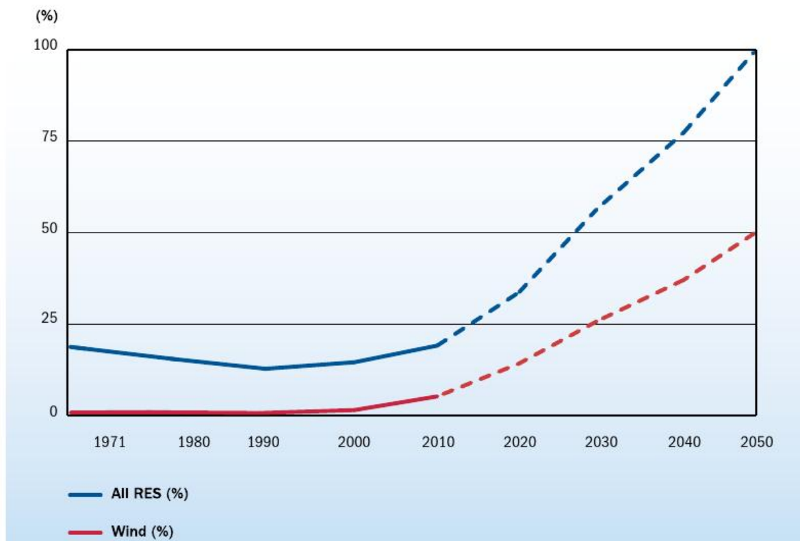
FIG 8: CONTRIBUTION OF ELECTRICITY FROM RENEWABLE ENERGY SOURCES AND WIND ENERGY 1970-2010 AND EXPECTED CONTRIBUTION 2011-2050 (% SHARE OF CONSUMPTION)
