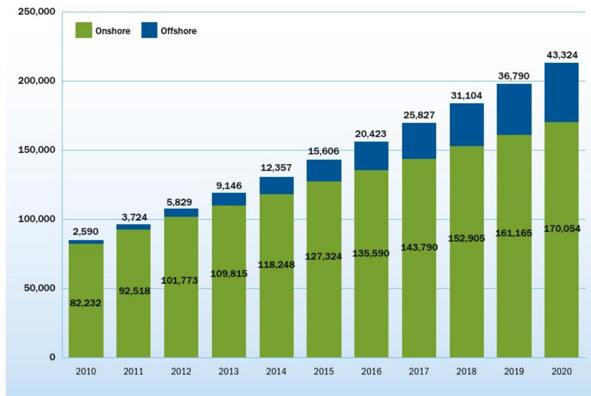
FIG 18: CUMULATIVE WIND POWER INSTALLATIONS IN THE EU (MW)
