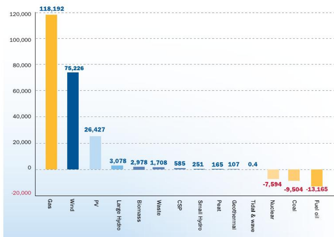
FIG 4: NET ELECTRICITY GENERATING INSTALLATIONS IN EU 2000 – 2010 (MW)
