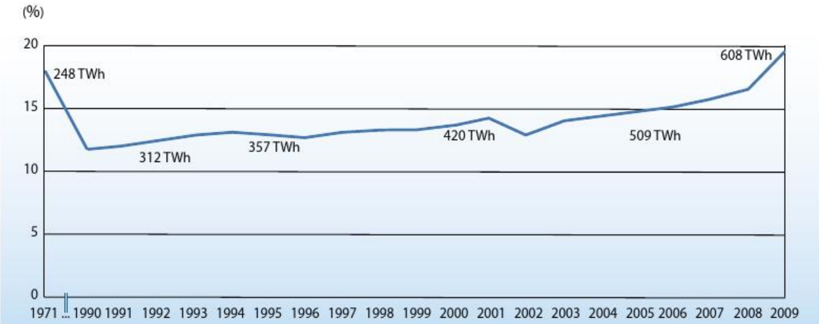
FIG 2: RENEWABLE ELECTRICITY'S SHARE OF TOTAL EU27 ELECTRICITY CONSUMPTION 1971 - 2010 (%)
