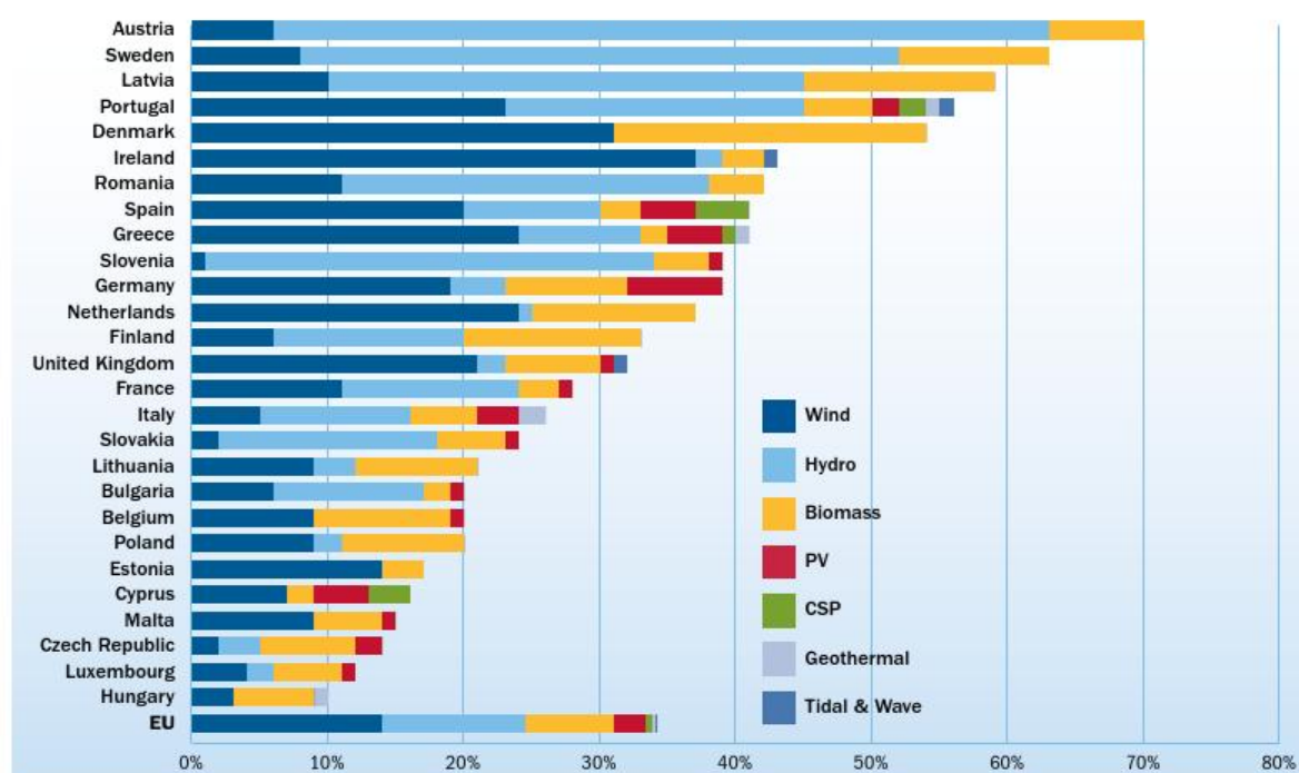
FIG 5: RENEWABLES' SHARE OF ELECTRICITY CONSUMPTION PER MEMBER STATE (%) IN 2020 ACCORDING TO THE NREAPS
