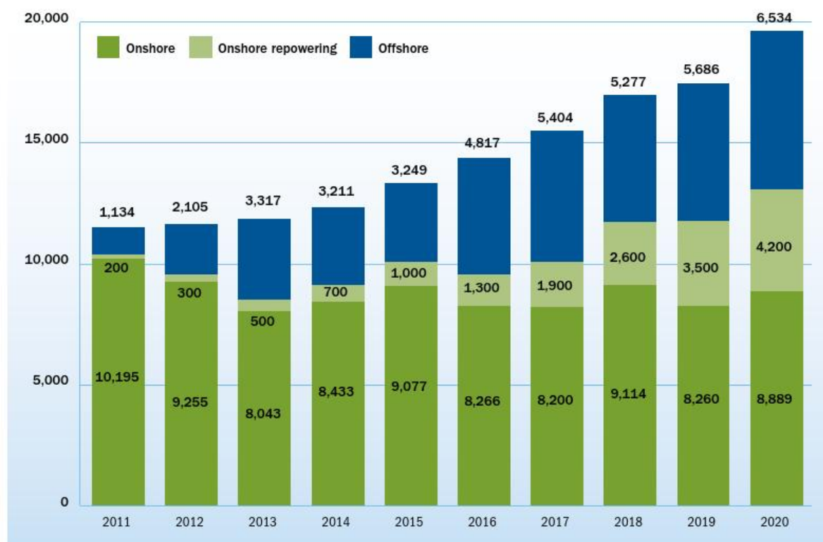
FIG 17: ESTIMATE OF THE TOTAL MARKET FOR WIND POWER 2011-2020 BROKEN DOWN BY ANNUAL NET ONSHORE AND OFFSHORE WIND POWER INSTALLATIONS IN THE EU AND EWEA ESTIMATE OF REPOWERING INSTALLATIONS IN THE EU (MW)
