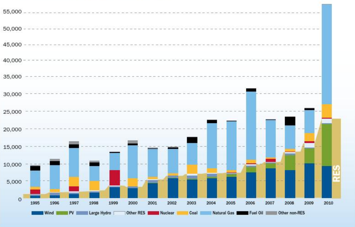
FIG 3: NEW INSTALLED CAPACITY PER YEAR 1995 - 2010 (MW)
